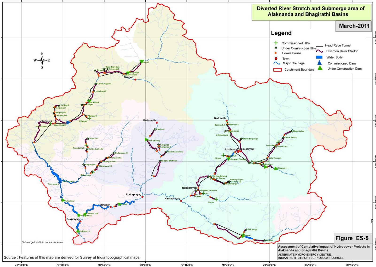
Fig. ES-5: All allotted projects with diversion and submergence of river Alaknanda and Bhagirathi Basins
